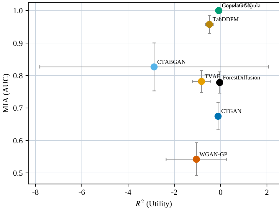
Metro Interstate: R^2 (Utility) vs MIA (AUC)
